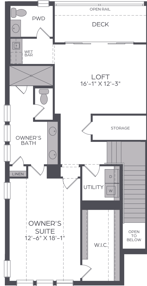
UPPER FLOOR
