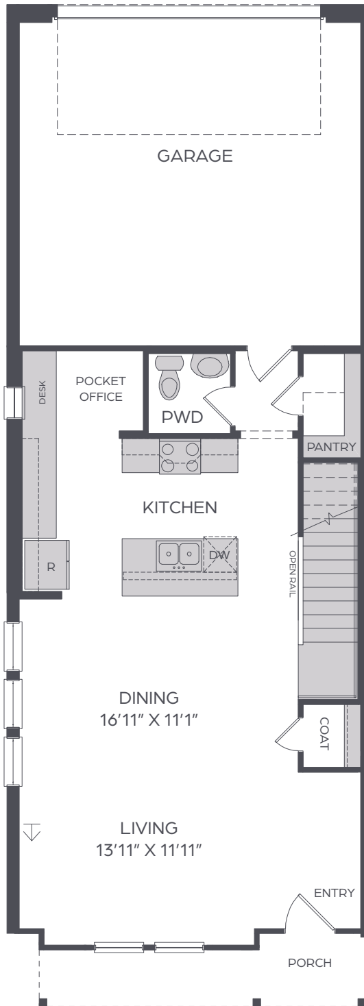
MAIN FLOOR
