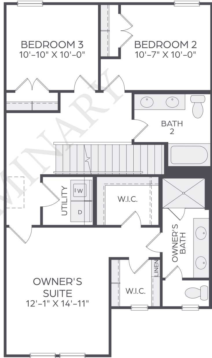
UPPER FLOOR
